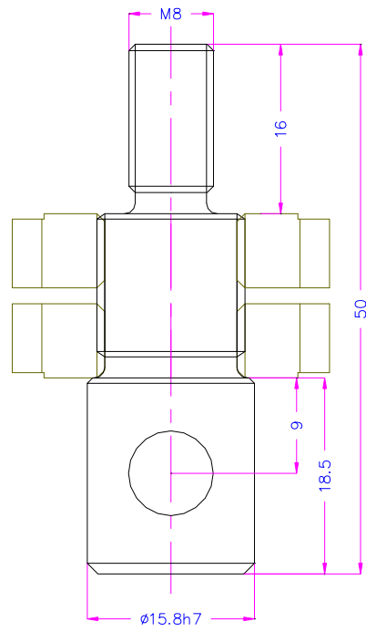
C45 Nickel THS464-158-M8 Adapter
